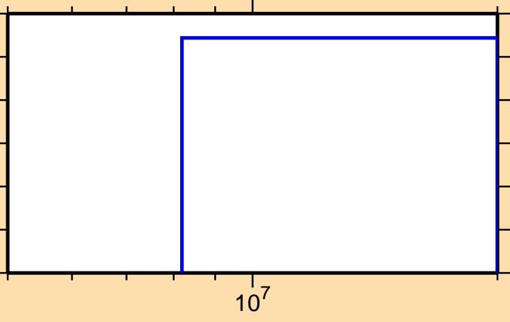
\sigma vs. E for ^{188}\text{Re}(n,2n\alpha)
