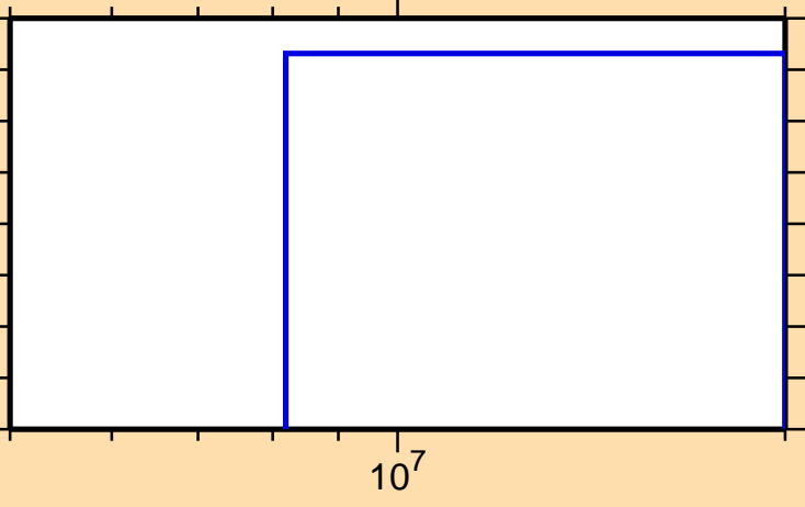
\sigma vs. E for ^{188}\text{Re}(n,nt)
