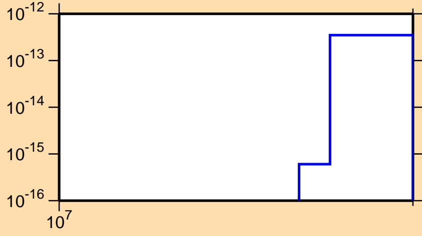
\sigma vs. E for ^{189}\text{Re}(n,\text{He3})
