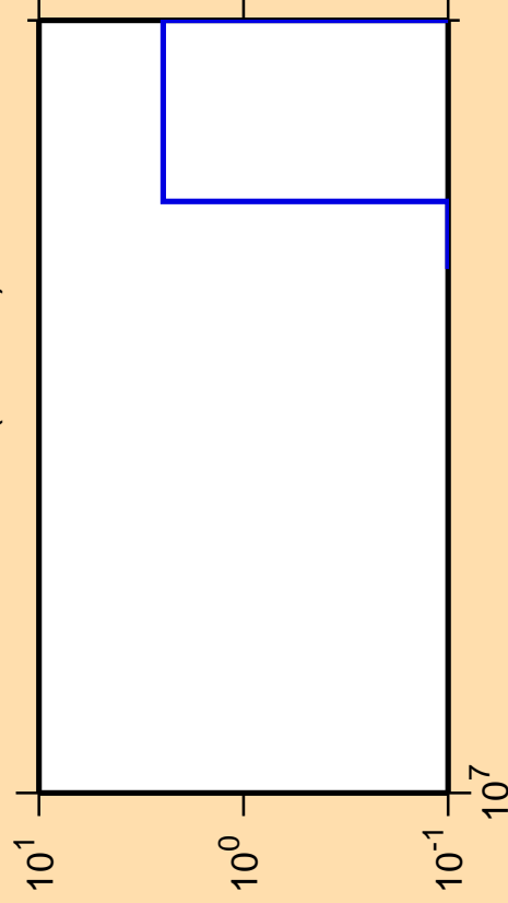
\Delta\sigma/\sigma vs. E for ^{189}\text{Re}(n,\text{He3})
