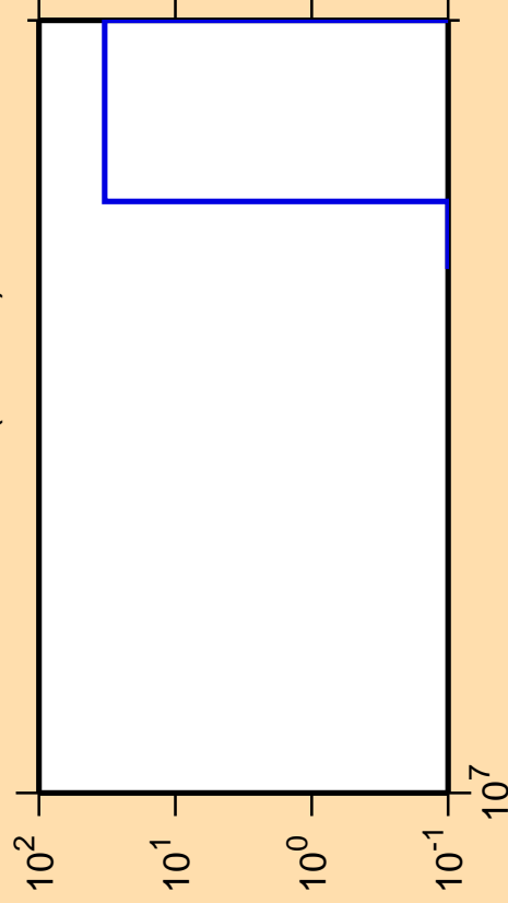
\Delta\sigma/\sigma vs. E for ^{189}\text{Re}(n,3n\alpha)
