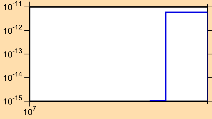
\sigma vs. E for ^{189}\text{Re}(n,3n\alpha)
