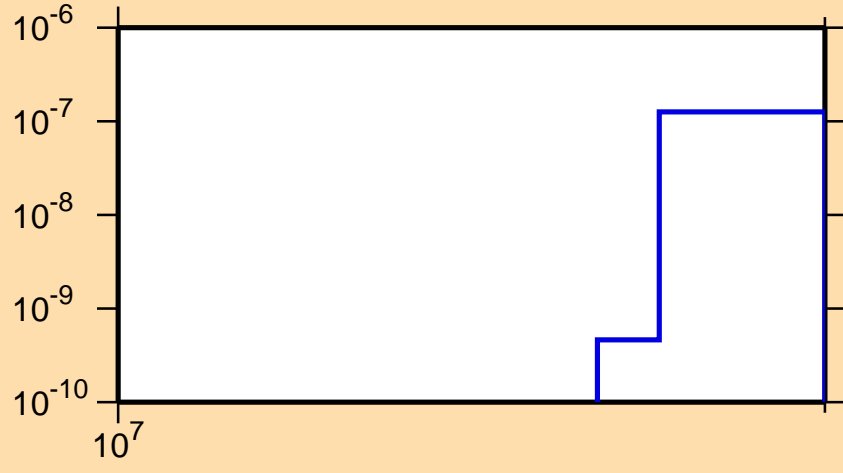
\sigma vs. E for ^{189}\text{Re}(n,2np)
