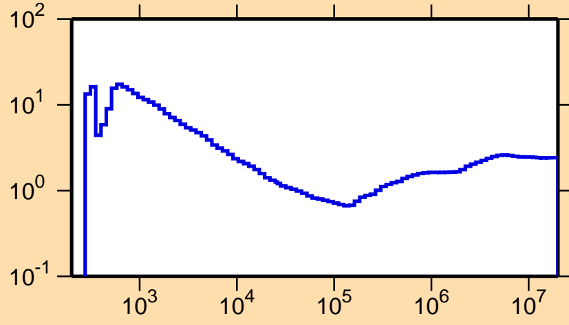
\sigma vs. E for ^{189}\text{Re}(n,\text{nonel.})
