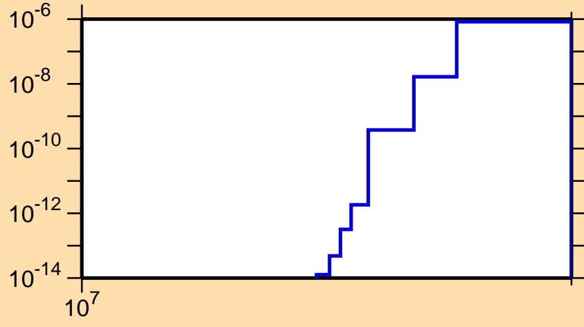
\sigma vs. E for ^{189}\text{Re}(n,\text{nd})
