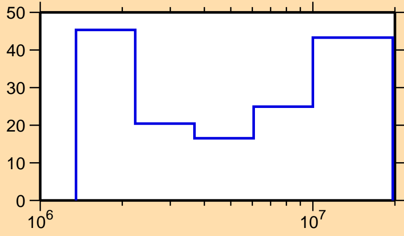
\Delta\sigma/\sigma vs. E for ^{189}\text{Re}(n,ncont.)
