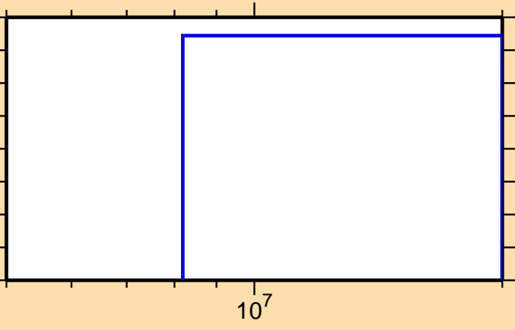
\sigma vs. E for ^{189}\text{Re}(n,\text{nd})
