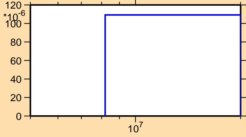
\sigma vs. E for ^{189}\text{Re}(n,np)
