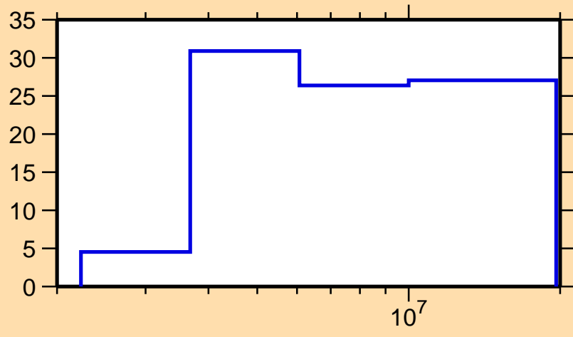
\Delta\sigma/\sigma vs. E for ^{190}\text{Re}(n,p)
