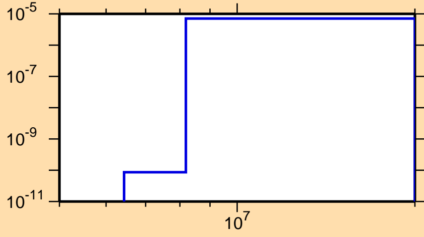
\sigma vs. E for ^{190}\text{Re}(n,n\alpha)
