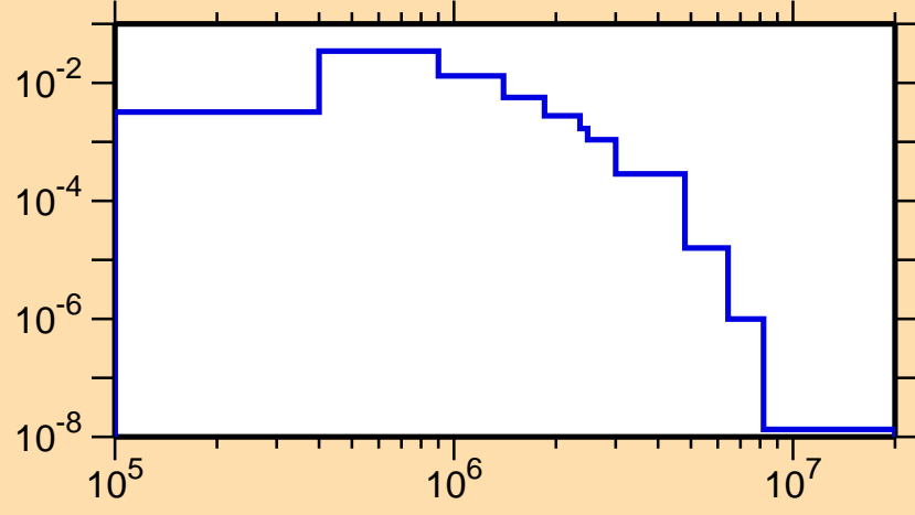
\sigma vs. E for ^{190}\text{Re}(n,n_4)
