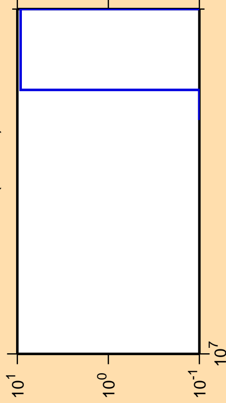
\Delta\sigma/\sigma vs. E for ^{190}\text{Re}(n,3n\alpha)
