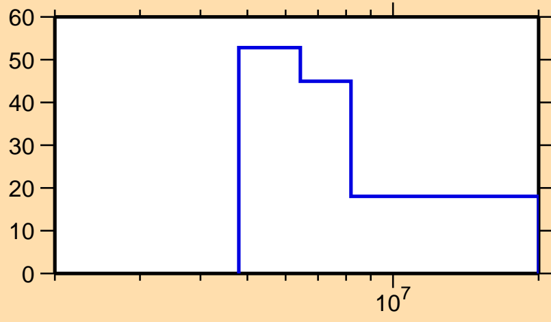
\Delta\sigma/\sigma vs. E for ^{190}\text{Re}(n,2n)
