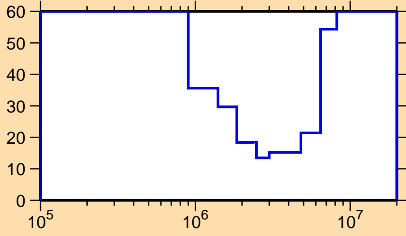
\Delta\sigma/\sigma vs. E for ^{190}\text{Re}(n,n\text{cont.})
