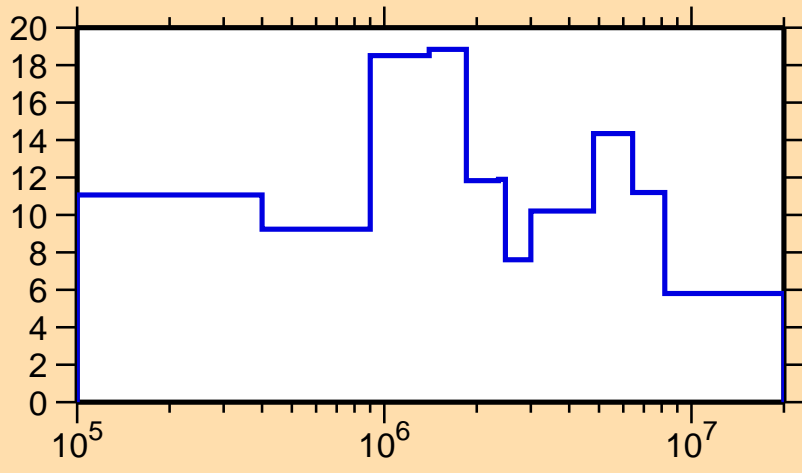
\Delta\sigma/\sigma vs. E for ^{190}\text{Re}(n, el.)
