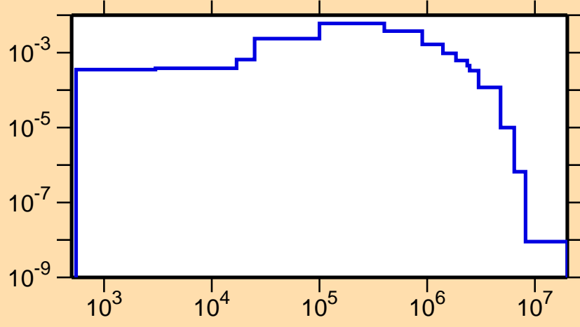
\sigma vs. E for ^{190}\text{Re}(n,n_1)
