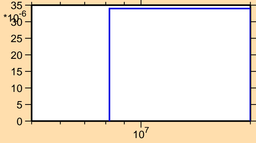
\sigma vs. E for ^{190}\text{Re}(n,t)
