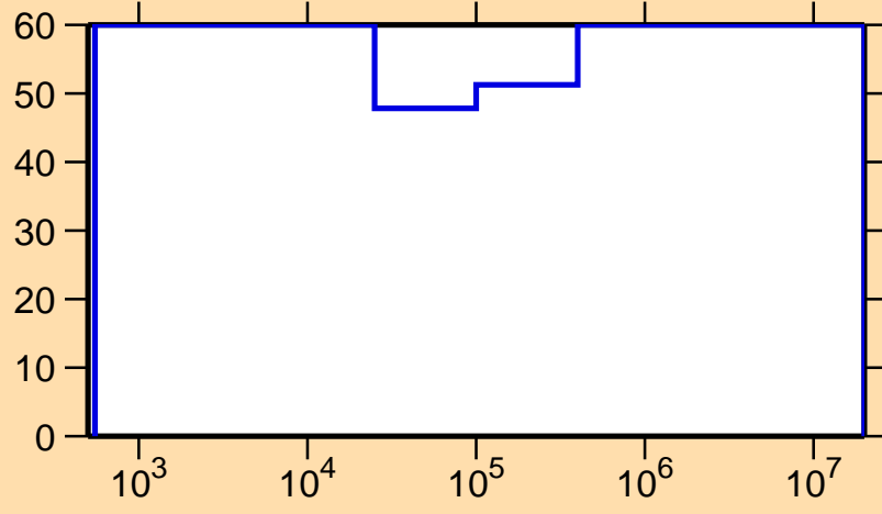
\Delta\sigma/\sigma vs. E for ^{190}\text{Re}(n,\gamma)
