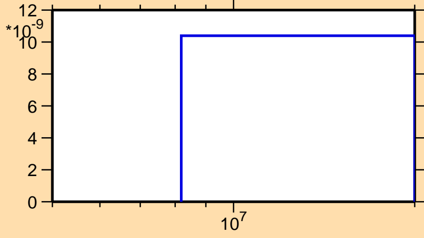
\sigma vs. E for ^{190}\text{Re}(n,2n\alpha)
