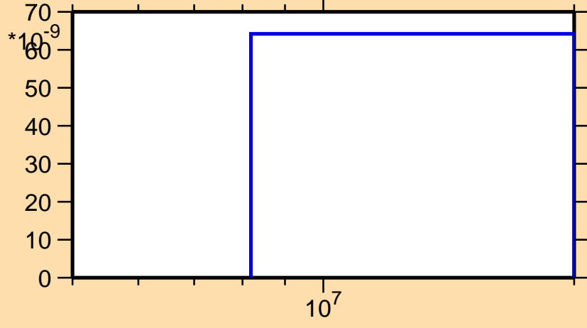
\sigma vs. E for ^{190}\text{Re}(n,\text{nd})
