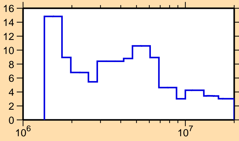
\Delta\sigma/\sigma vs. E for ^{191}\text{Re}(n, el.)
