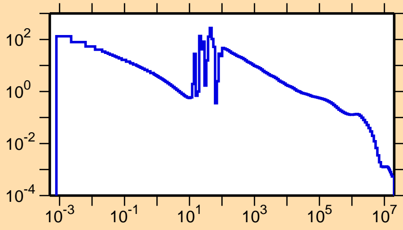
\sigma vs. E for ^{191}\text{Re}(n,\gamma)
