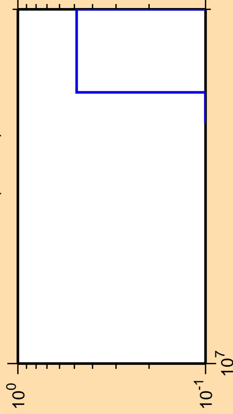
\Delta\sigma/\sigma vs. E for ^{191}\text{Re}(n,3n\alpha)
