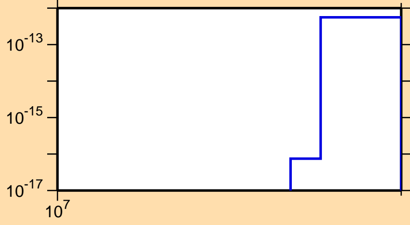
\sigma vs. E for ^{191}\text{Re}(n,3n\alpha)
