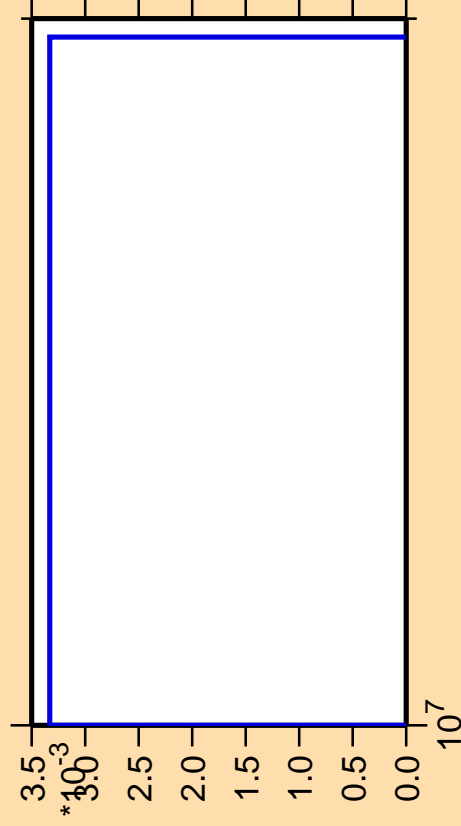
\Delta\sigma/\sigma vs. E for ^{191}\text{Re}(n,3n\alpha)
