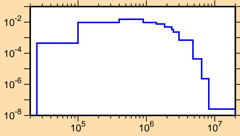
\sigma vs. E for ^{191}\text{Re}(n,n_1)
