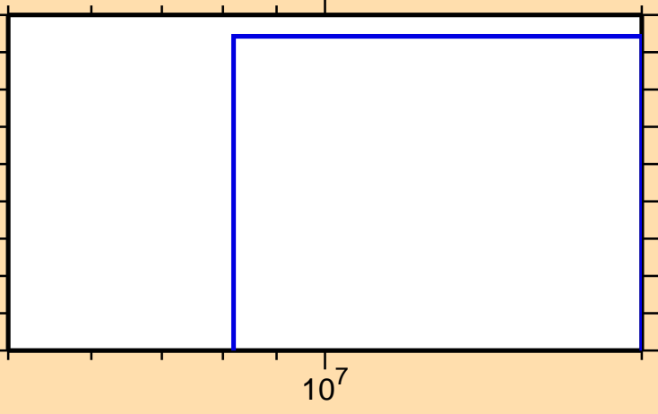
\sigma vs. E for ^{191}\text{Re}(n,\text{nd})
