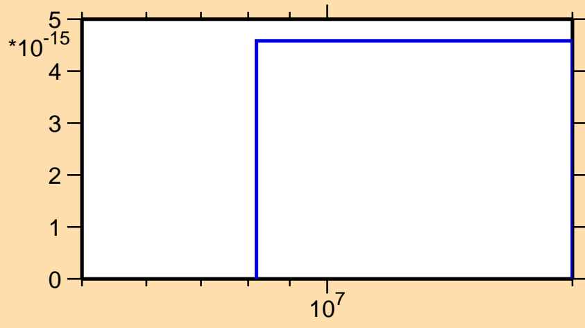
\sigma vs. E for ^{191}\text{Re}(n,3n\alpha)
