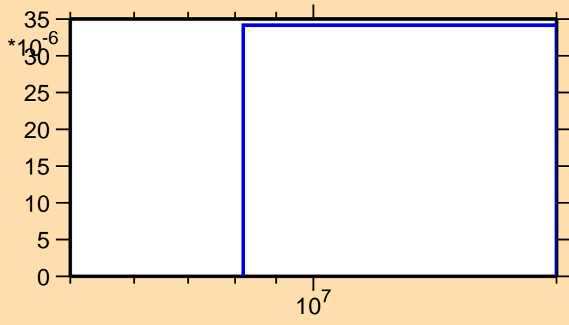
\sigma vs. E for ^{191}\text{Re}(n,np)
