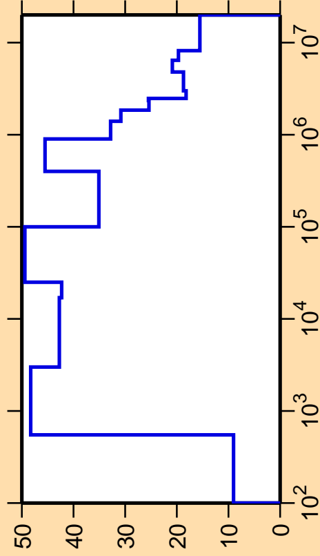
\Delta\sigma/\sigma vs. E for ^{192}\text{Re}(n,\text{nonel.})
