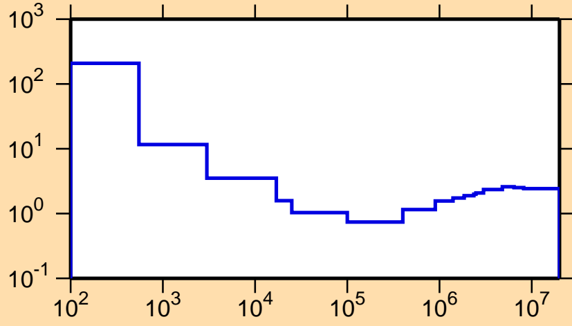
\sigma vs. E for ^{192}\text{Re}(n,\text{nonel.})
