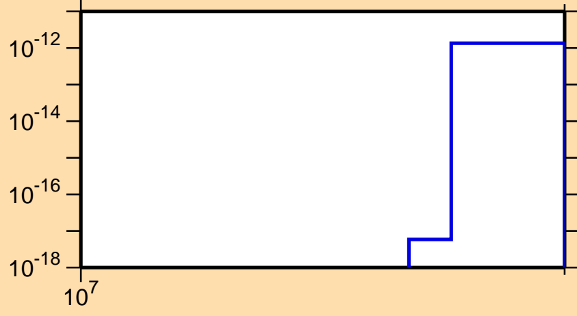
\sigma vs. E for ^{192}\text{Re}(n,3n\alpha)
