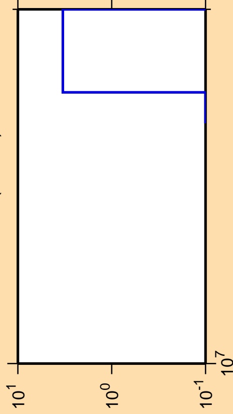
\Delta\sigma/\sigma vs. E for ^{192}\text{Re}(n,3n\alpha)
