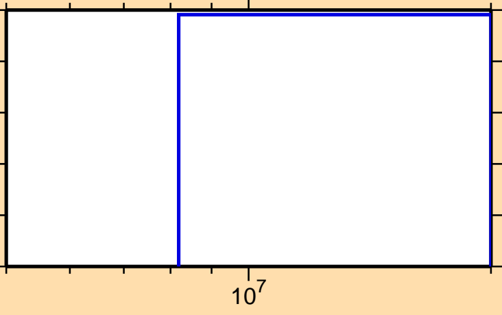
\sigma vs. E for ^{192}\text{Re}(n,\text{nd})
