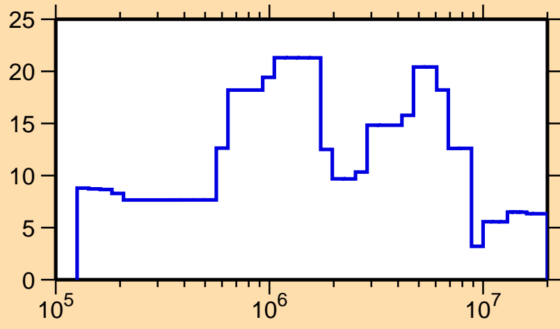
\Delta\sigma/\sigma vs. E for ^{193}\text{Re}(n,\text{el.})
