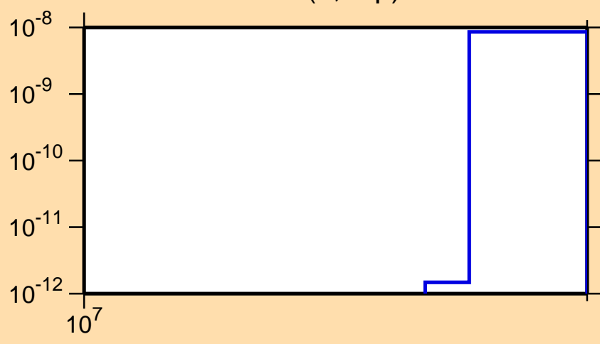
\sigma vs. E for ^{193}\text{Re}(n,2np)
