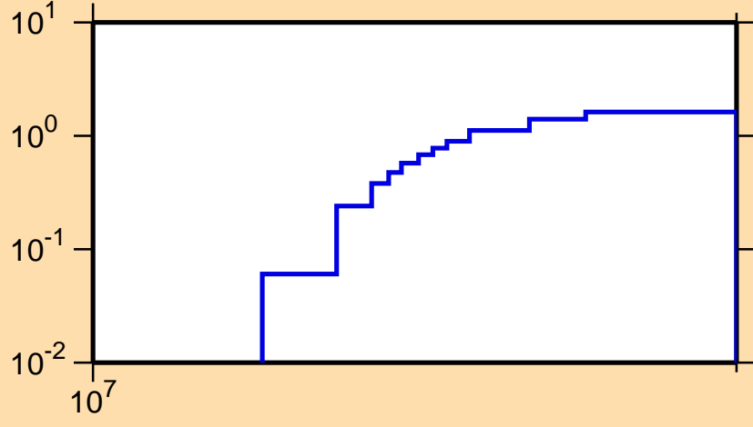
\sigma vs. E for ^{193}\text{Re}(n,3n)
