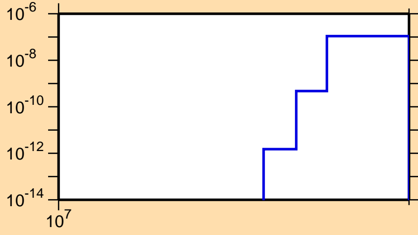
\sigma vs. E for ^{193}\text{Re}(n,\text{nd})
