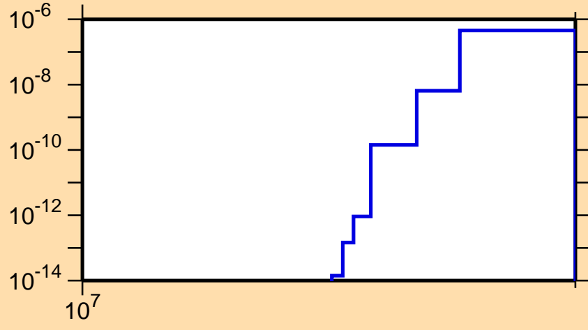
\sigma vs. E for ^{193}\text{Re}(n,nt)
