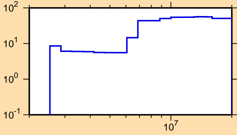
\Delta\sigma/\sigma vs. E for ^{193}\text{Re}(n,n\text{cont.})
