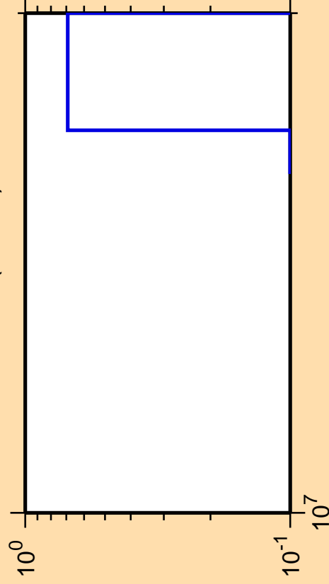
\Delta\sigma/\sigma vs. E for ^{193}\text{Re}(n,3n\alpha)
