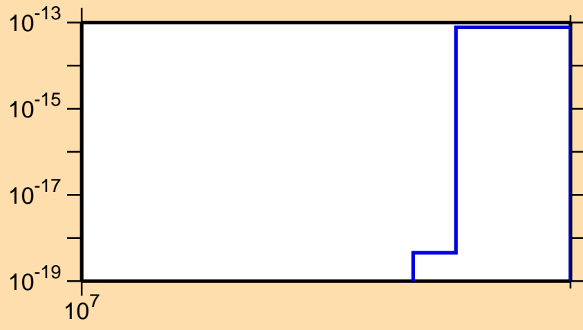
\sigma vs. E for ^{193}\text{Re}(n,3n\alpha)
