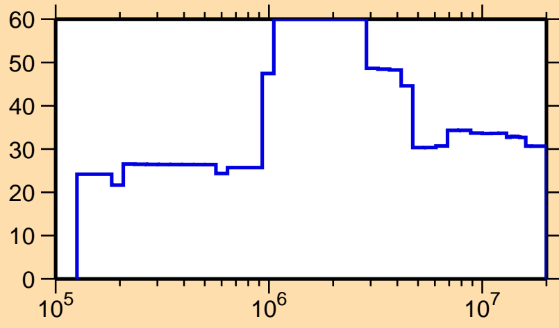
\Delta\sigma/\sigma vs. E for ^{193}\text{Re}(n,n_1)
