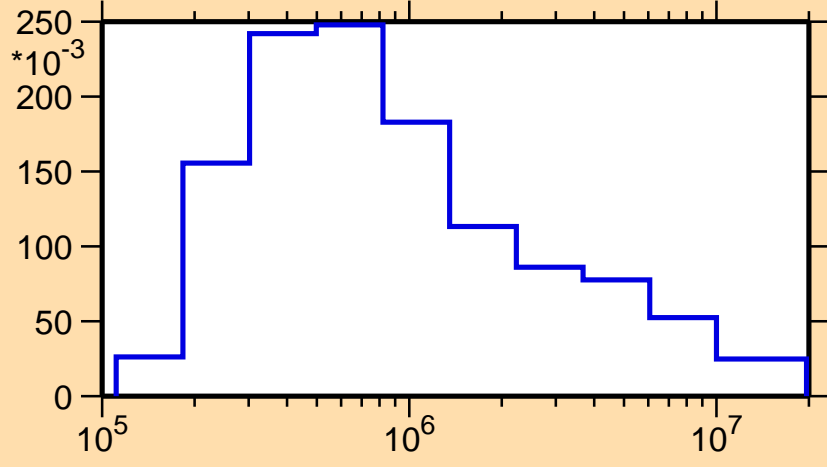
\sigma vs. E for ^{193}\text{Re}(n,n_1)
