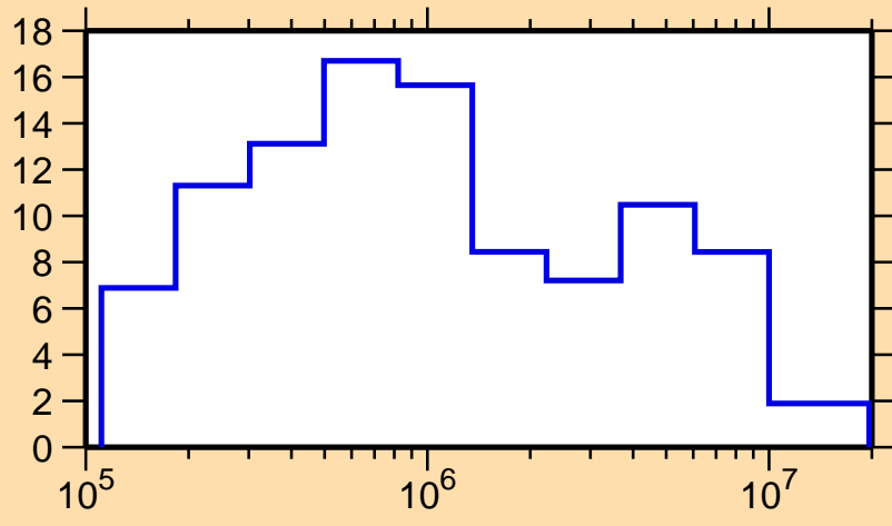
\Delta\sigma/\sigma vs. E for ^{193}\text{Re}(n,\text{tot.})
