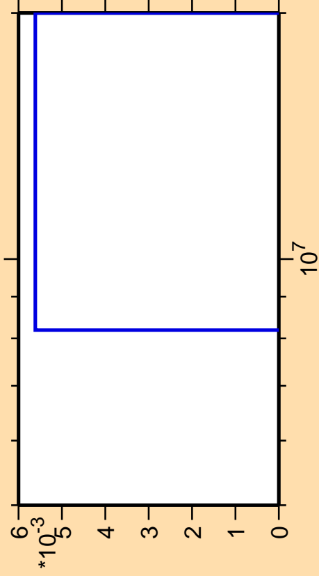
\Delta\sigma/\sigma vs. E for ^{193}\text{Re}(n,3n\alpha)
