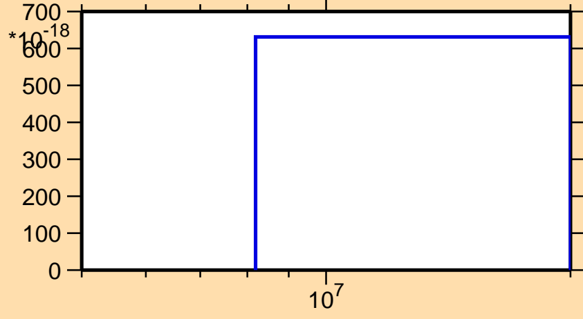
\sigma vs. E for ^{193}\text{Re}(n,3n\alpha)
