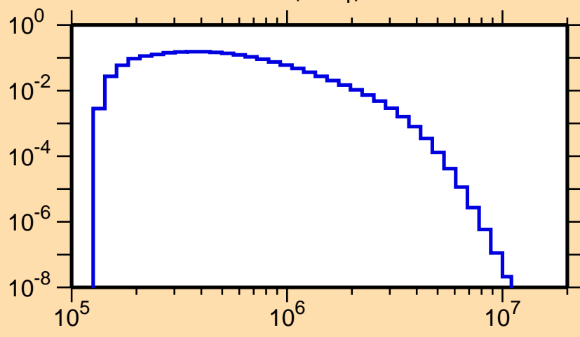
\sigma vs. E for ^{194}\text{Re}(n,n_1)
