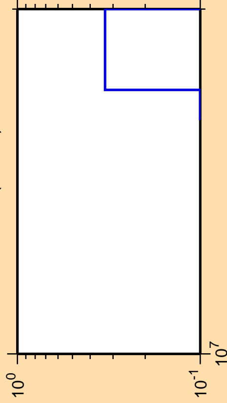
\Delta\sigma/\sigma vs. E for ^{194}\text{Re}(n,3n\alpha)
