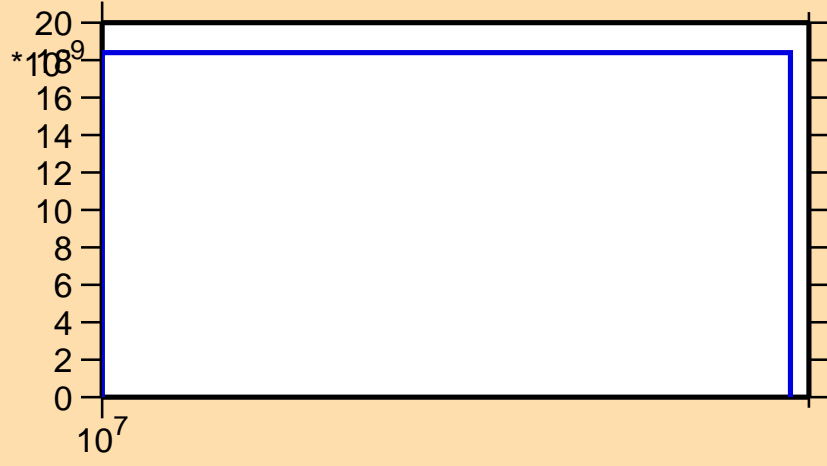
\sigma vs. E for ^{194}\text{Re}(n,\text{nd})
