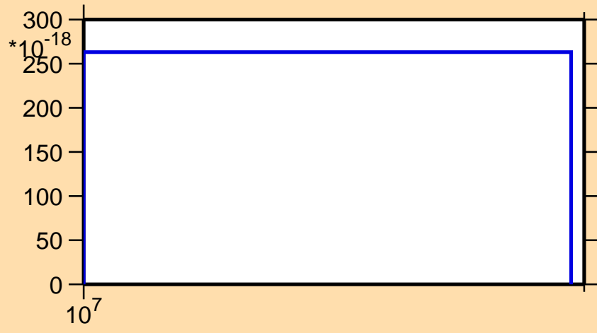
\sigma vs. E for ^{194}\text{Re}(n,3n\alpha)
