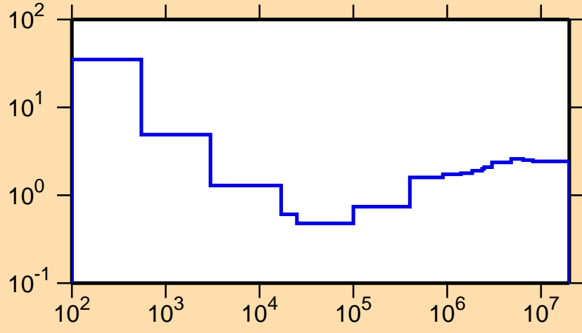
\sigma vs. E for ^{194}\text{Re}(n,\text{nonel.})
