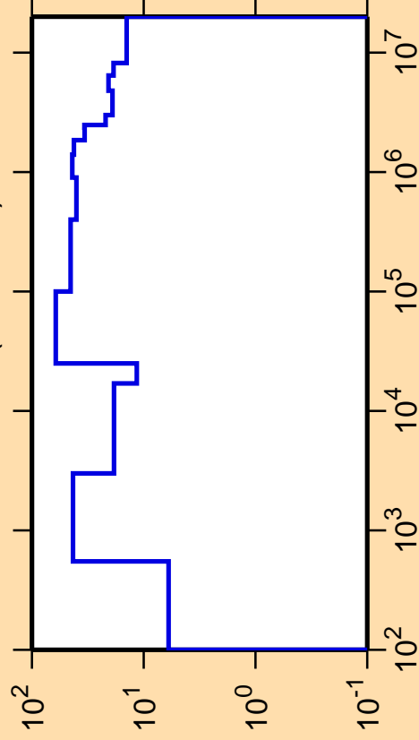
\Delta\sigma/\sigma vs. E for ^{194}\text{Re}(n,\text{nonel.})
