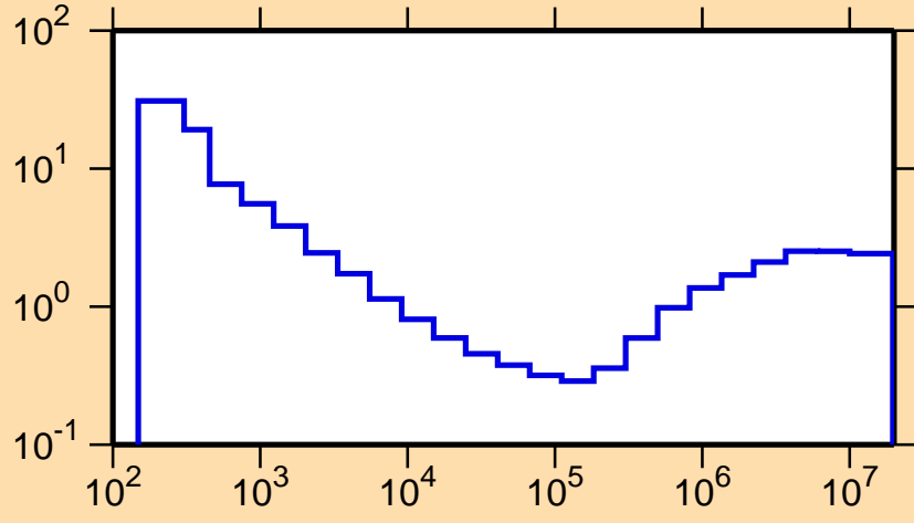
\sigma vs. E for ^{195}\text{Re}(n,\text{nonel.})
