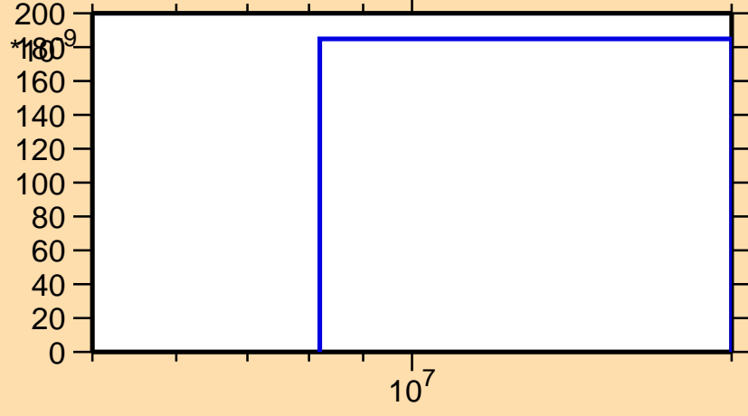
\sigma vs. E for ^{195}\text{Re}(n,n\alpha)
