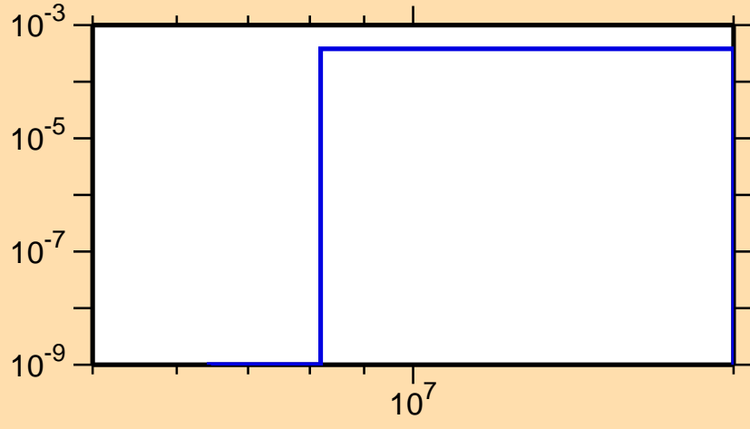
\sigma vs. E for ^{195}\text{Re}(n,p)
