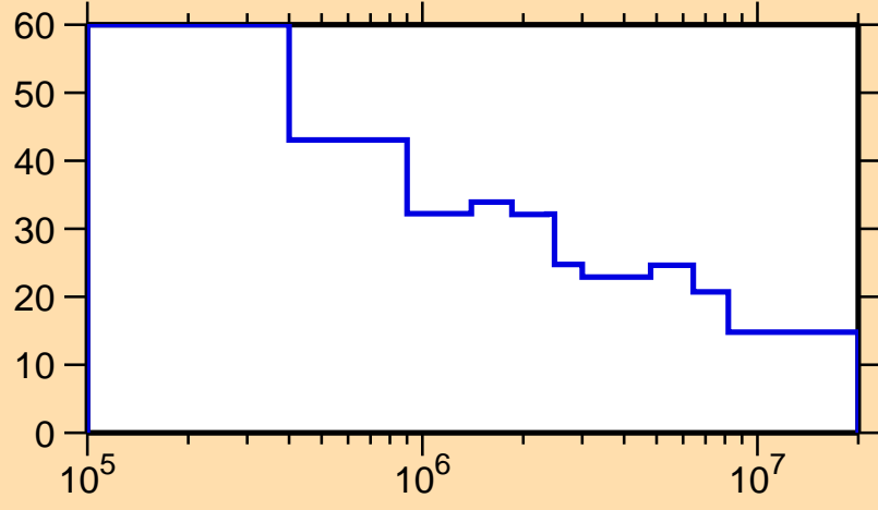
\Delta\sigma/\sigma vs. E for ^{195}\text{Re}(n,n\text{onel.})
