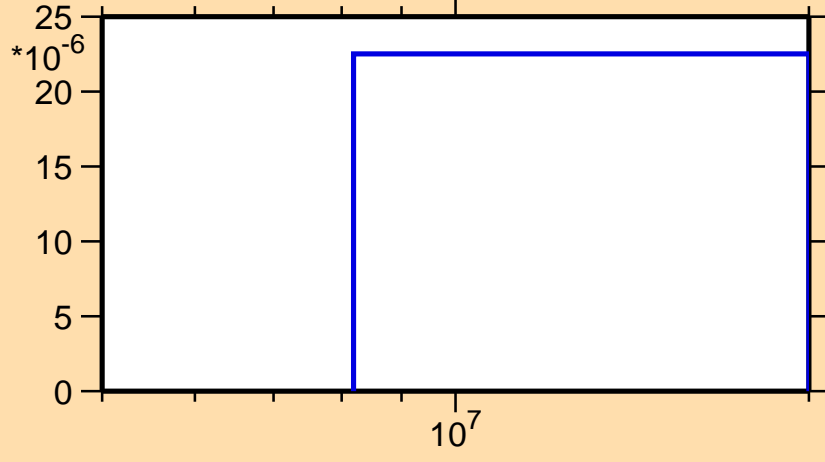
\sigma vs. E for ^{195}\text{Re}(n,np)
