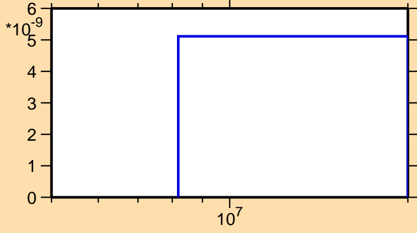
\sigma vs. E for ^{196}\text{Re}(n,nt)
