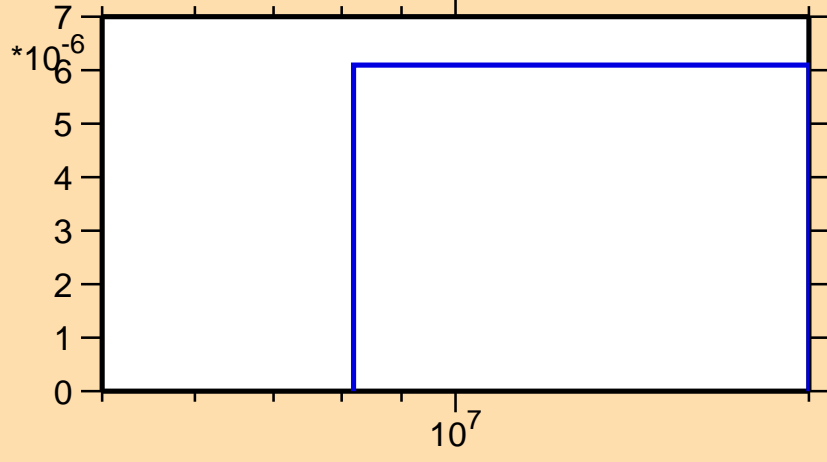
\sigma vs. E for ^{196}\text{Re}(n,t)
