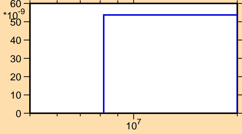
\sigma vs. E for ^{196}\text{Re}(n,n\alpha)
