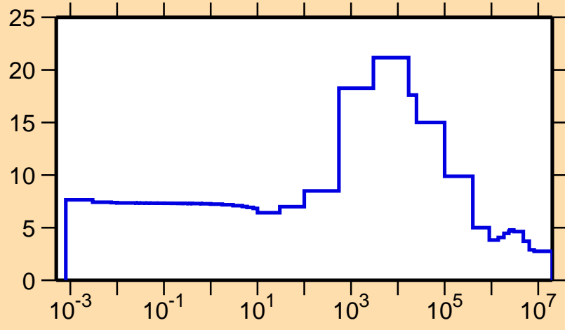
\sigma vs. E for ^{196}\text{Re}(n,\text{el.})
