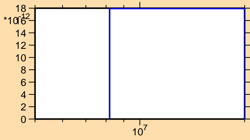
\sigma vs. E for ^{196}\text{Re}(n,2n\alpha)
