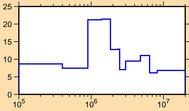
\Delta\sigma/\sigma vs. E for ^{196}\text{Re}(n, el.)
