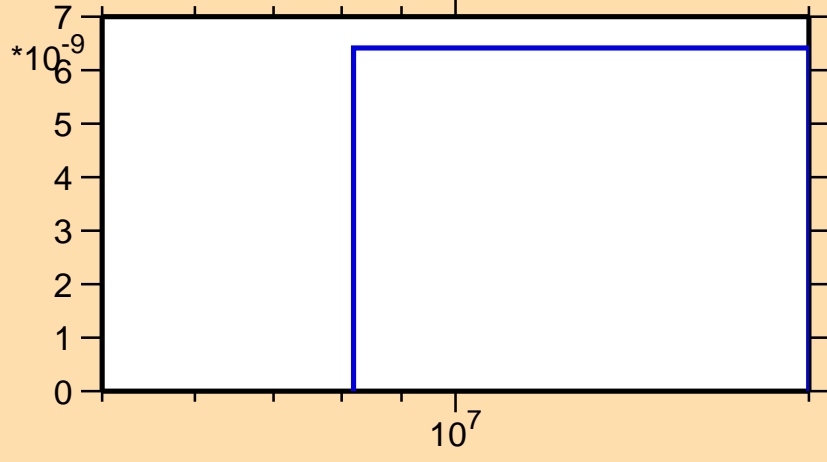
\sigma vs. E for ^{196}\text{Re}(n,\text{nd})
