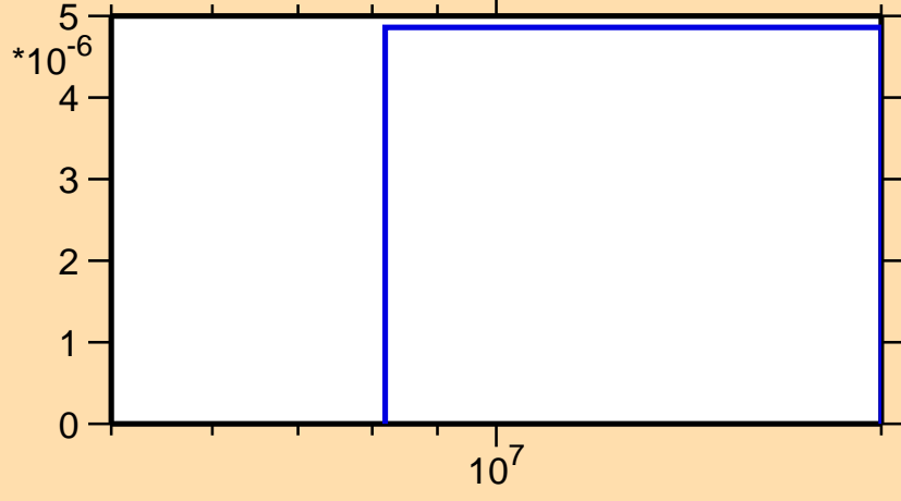
\sigma vs. E for ^{196}\text{Re}(n,np)
