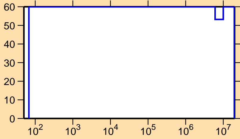
\Delta\sigma/\sigma vs. E for ^{255}\gamma
