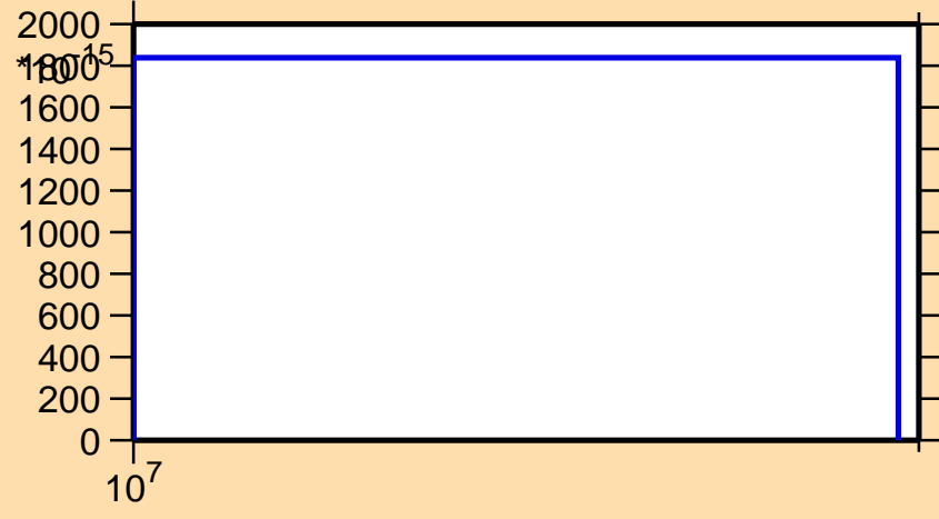
\sigma vs. E for ^{255}
