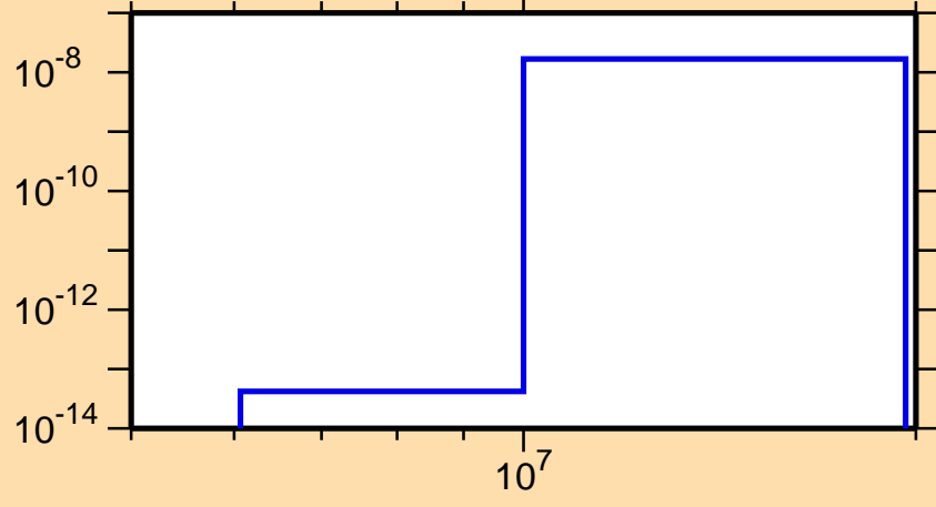
\sigma vs. E for ^{255}\text{He3}
