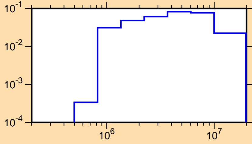
\sigma vs. E for ^{255}\alpha
