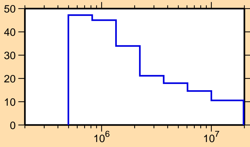
\Delta\sigma/\sigma vs. E for 255
