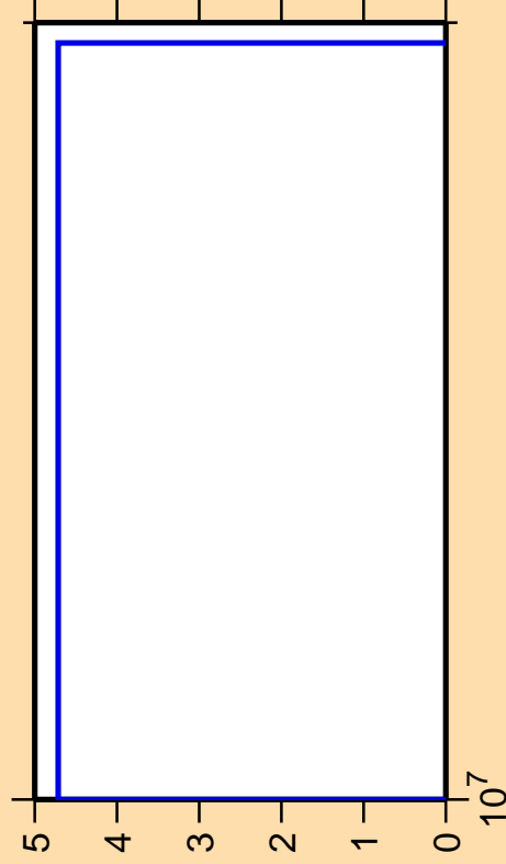
\Delta\sigma/\sigma vs. E for ^{255}
