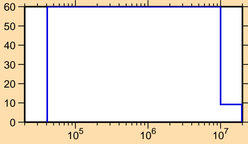
\Delta\sigma/\sigma vs. E for ^{255}_{1}\text{Po}
