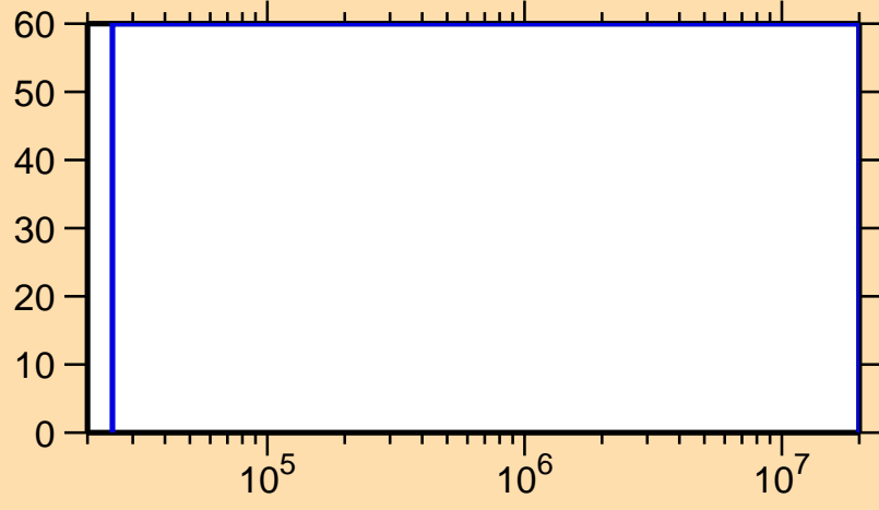
\Delta\sigma/\sigma vs. E for ^{255}_{1}\text{Pa}
