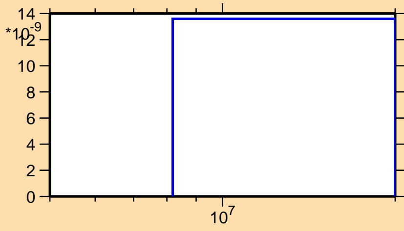
\sigma vs. E for ^{255}\text{He3}
