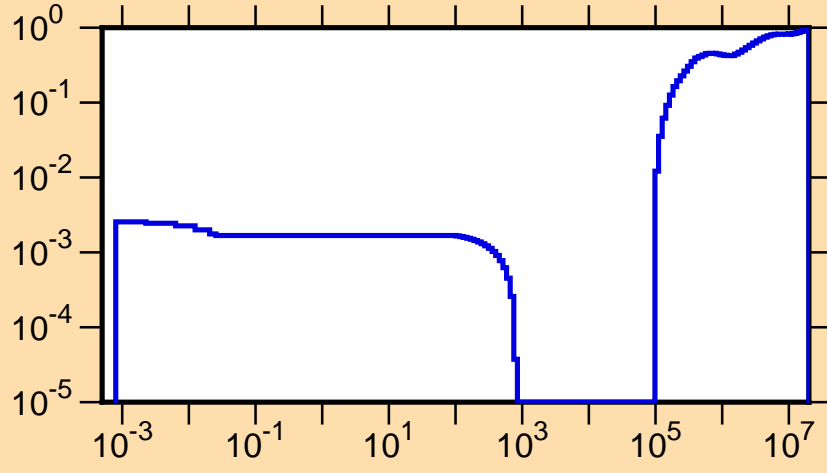
\mu vs. E for ^{257}
