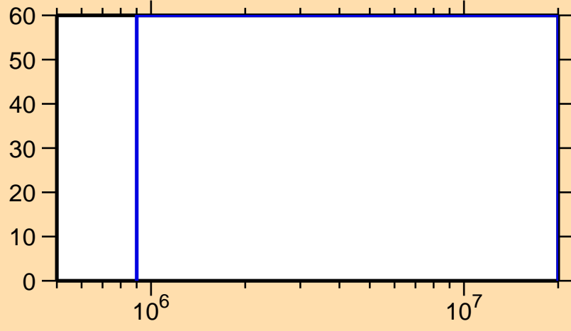
\Delta\sigma/\sigma vs. E for ^{257}_{1}\text{Pu}
