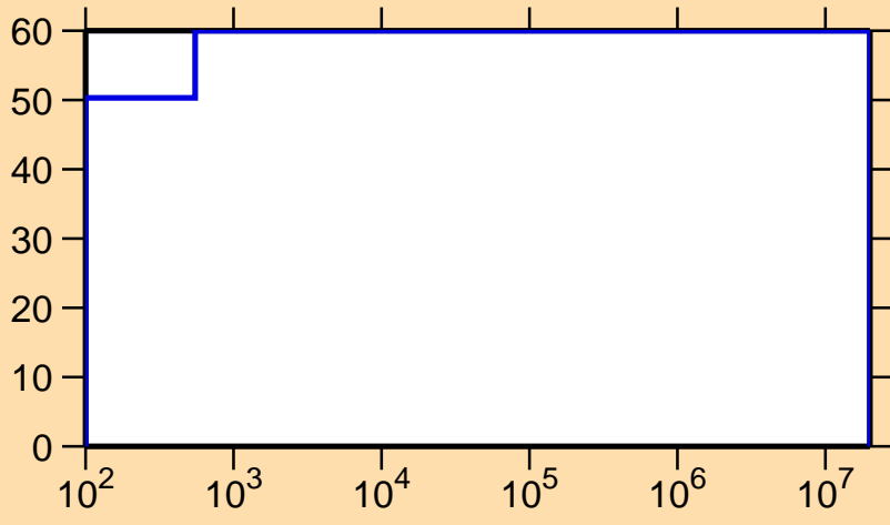
\Delta\sigma/\sigma vs. E for ^{257}\gamma
