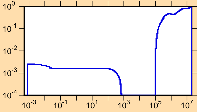
\mu vs. E for ^{259}
