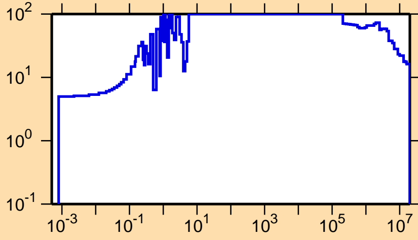
\Delta\sigma/\sigma vs. E for ^{259}\text{Pa}
