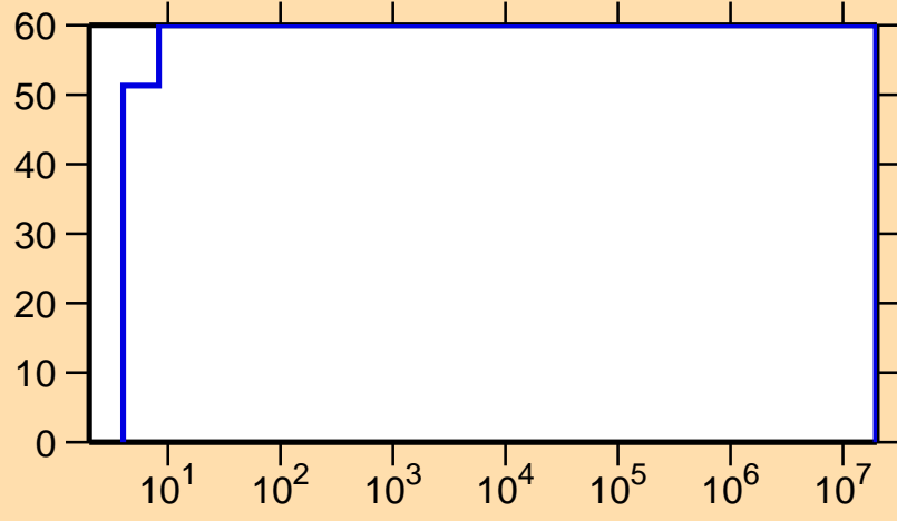
\Delta\sigma/\sigma vs. E for ^{259}\gamma
