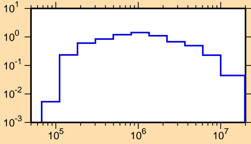
\sigma vs. E for 259
