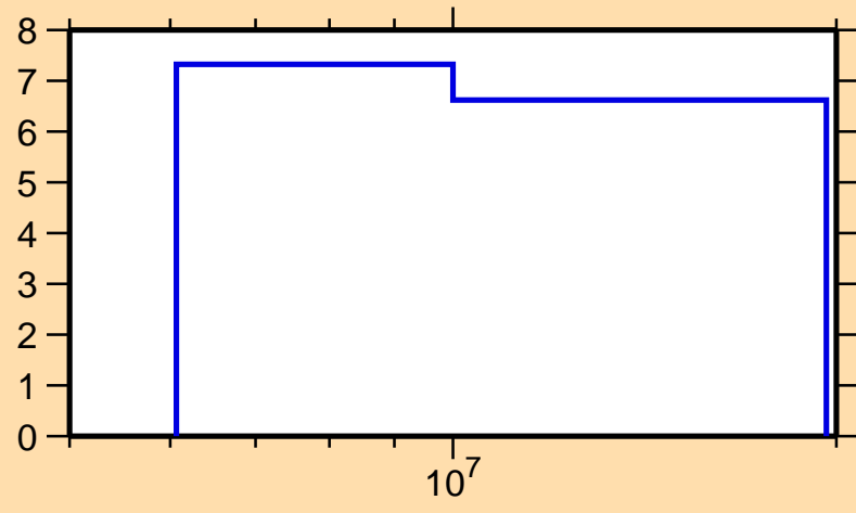
\Delta\sigma/\sigma vs. E for 259
