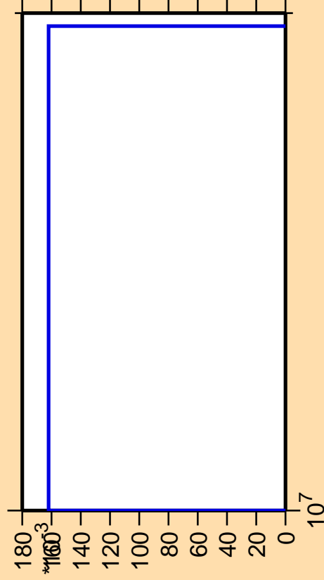
\Delta\sigma/\sigma vs. E for ^{259}
