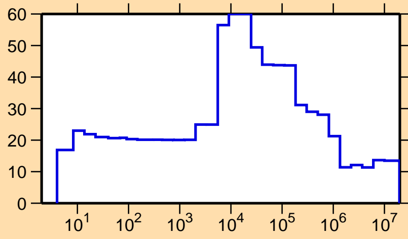
\Delta\sigma/\sigma vs. E for ^{259}
