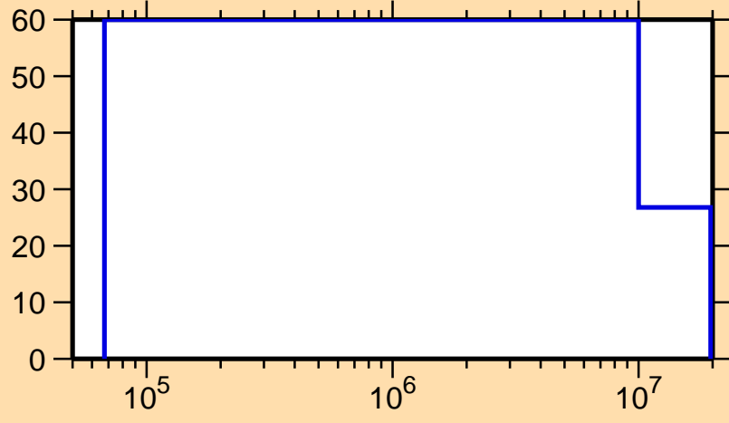
\Delta\sigma/\sigma vs. E for ^{259}_{1}
