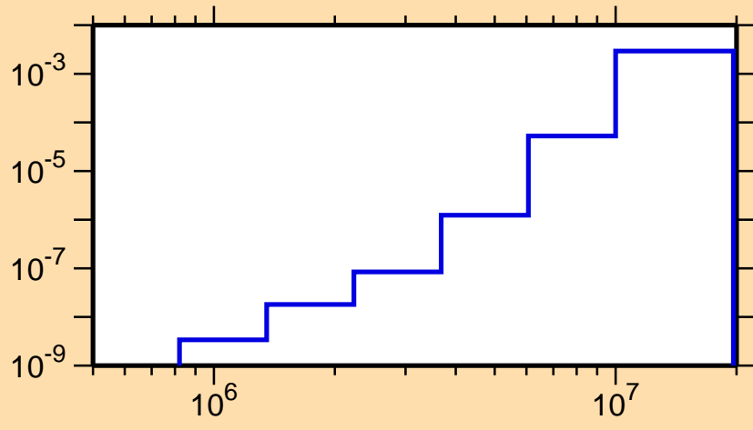
\sigma vs. E for ^{259}\alpha
