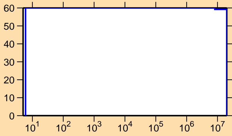
\Delta\sigma/\sigma vs. E for ^{259}\gamma
