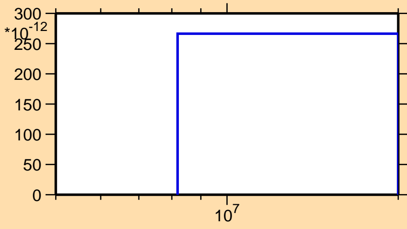
\sigma vs. E for ^{259}\text{He3}
