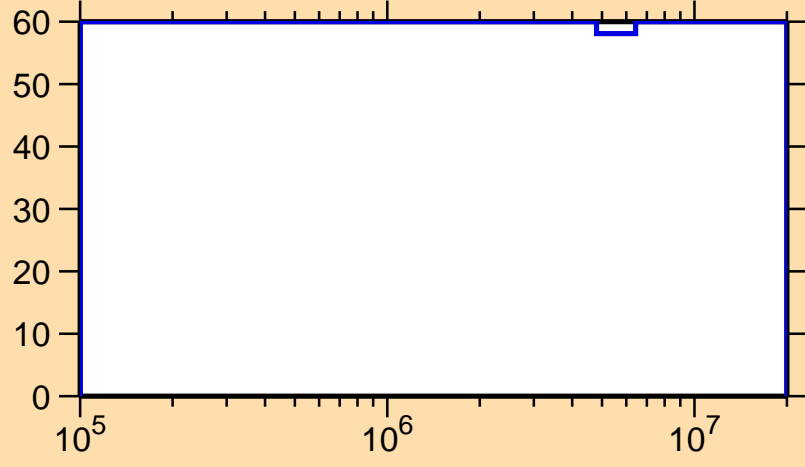
\Delta\sigma/\sigma vs. E for ^{259}\text{Pu}
