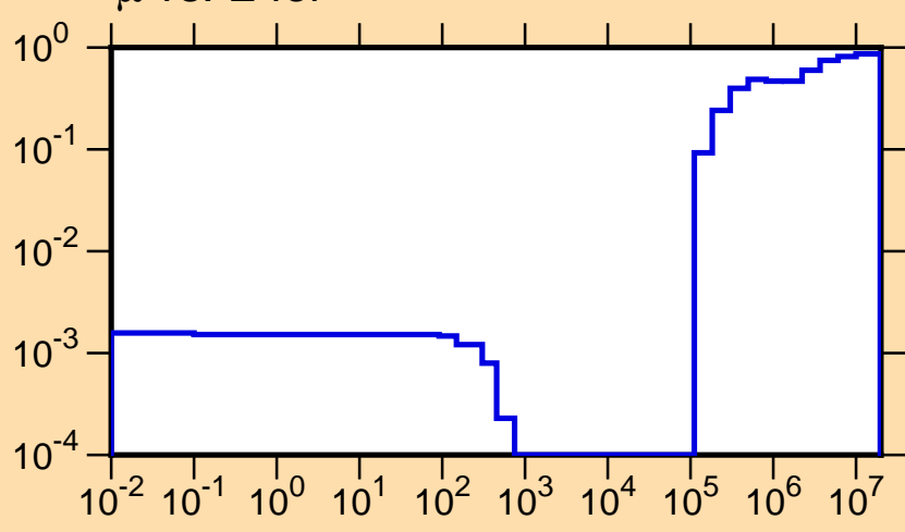
\mu vs. E for ^{261}
