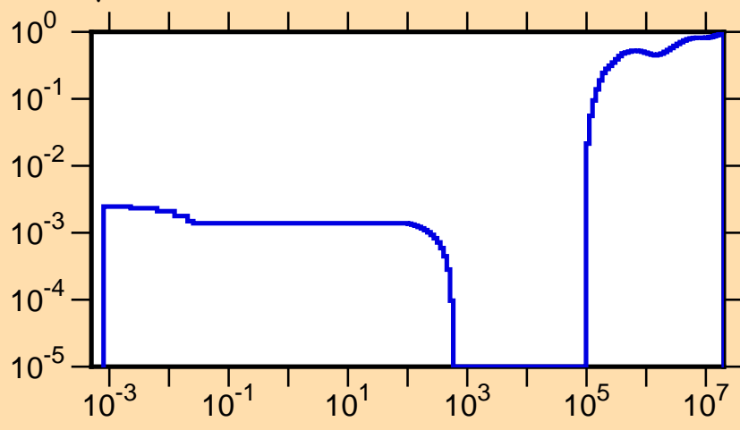
\mu vs. E for ^{265}
