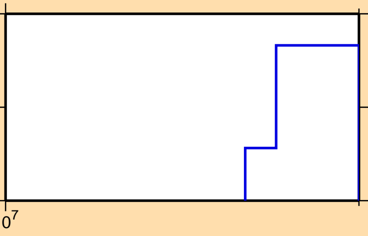
\sigma vs. E for ^{266}\text{He3}
