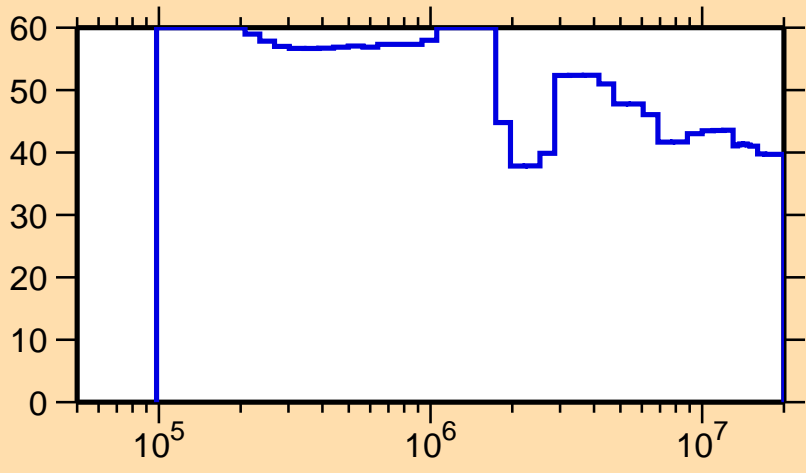
\Delta\sigma/\sigma vs. E for ^{267}_1
