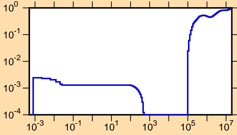
\mu vs. E for ^{268}
