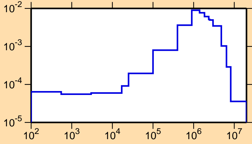
\sigma vs. E for ^{91}\text{Rh}(n,\text{inel.})
