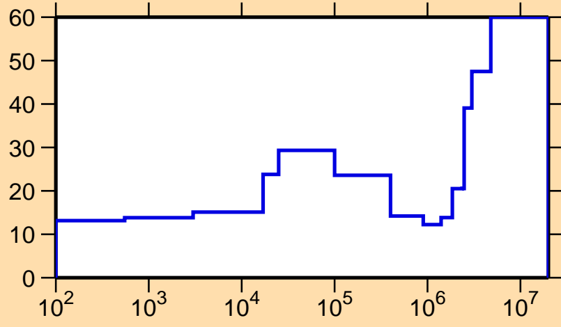
\Delta\sigma/\sigma vs. E for ^{91}\text{Rh}(n,p)
