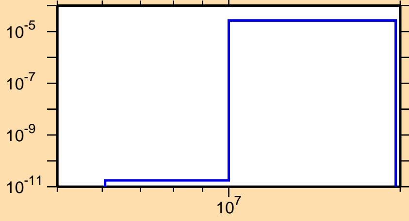
\sigma vs. E for ^{92}\text{Rh}(n,n\alpha)
