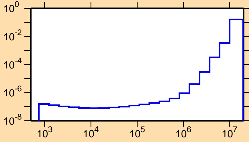
\sigma vs. E for ^{92}\text{Rh}(n,p\alpha)
