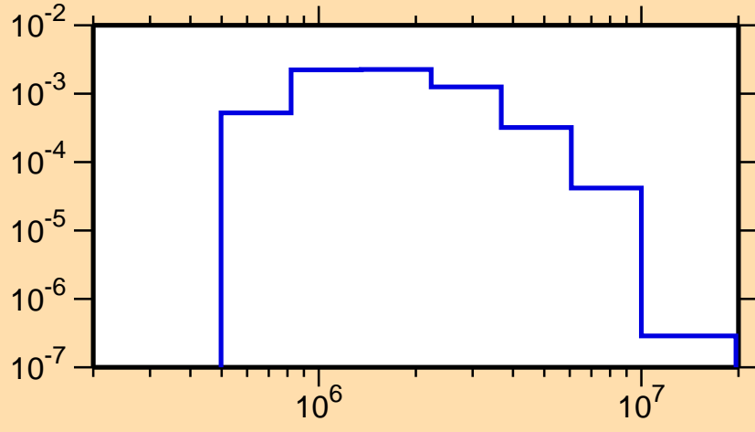
\sigma vs. E for ^{92}\text{Rh}(n,n_2)
