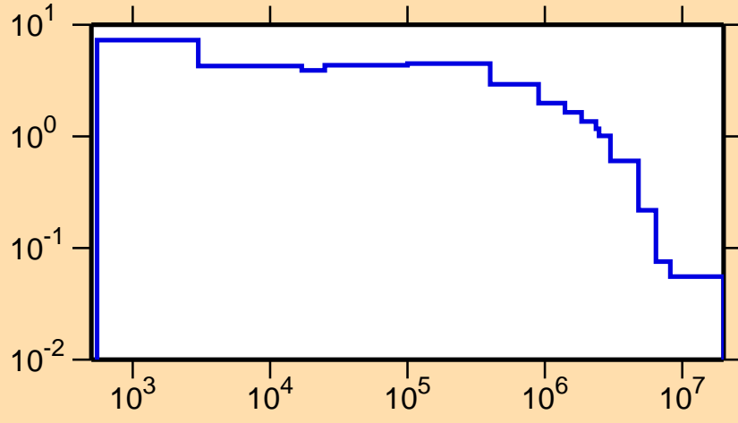
\sigma vs. E for ^{92}\text{Rh}(n,p)
