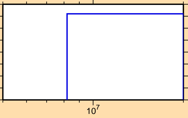
\sigma vs. E for ^{92}\text{Rh}(n,2n)
