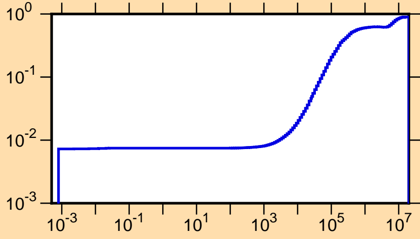
\mu vs. E for ^{93}\text{Rh}(\text{mt251})
