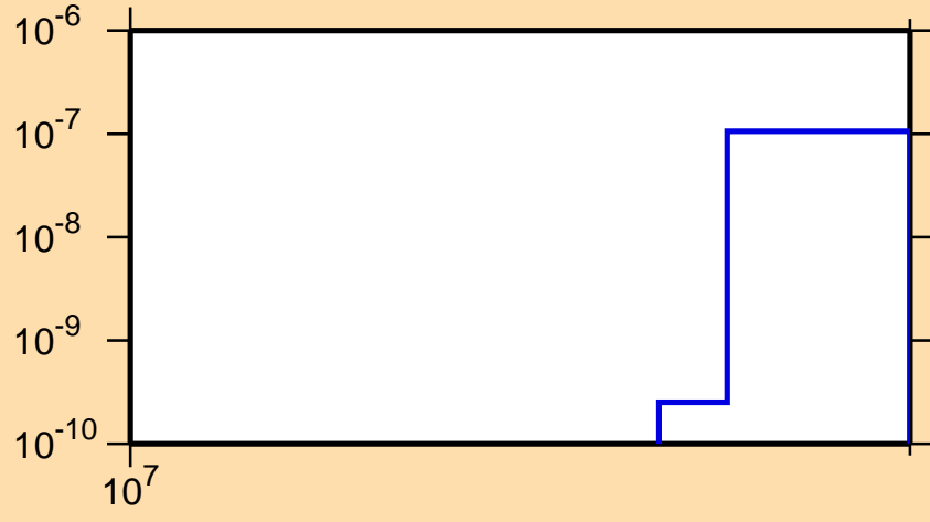
\sigma vs. E for ^{93}\text{Rh}(n,\text{nd})
