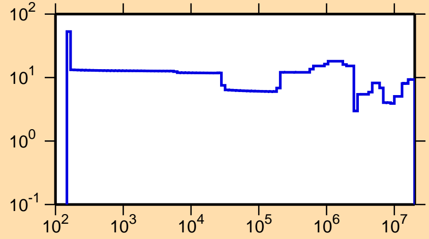
\Delta\sigma/\sigma vs. E for ^{93}\text{Rh}(n,\text{el.})
