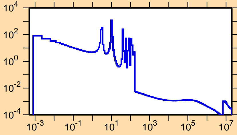
\sigma vs. E for ^{93}\text{Rh}(n,\gamma)
