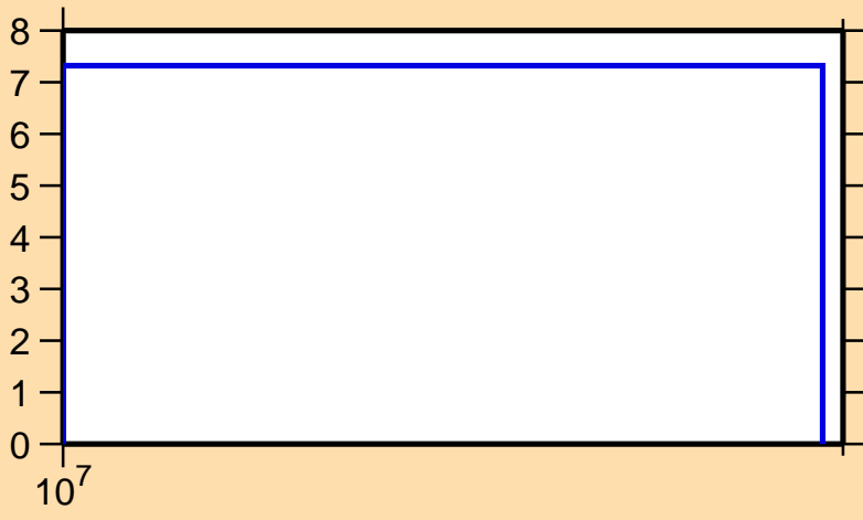
\Delta\sigma/\sigma vs. E for ^{93}\text{Rh}(n,\text{el.})
