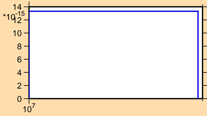
\sigma vs. E for ^{93}\text{Rh}(\text{mt } 34)
