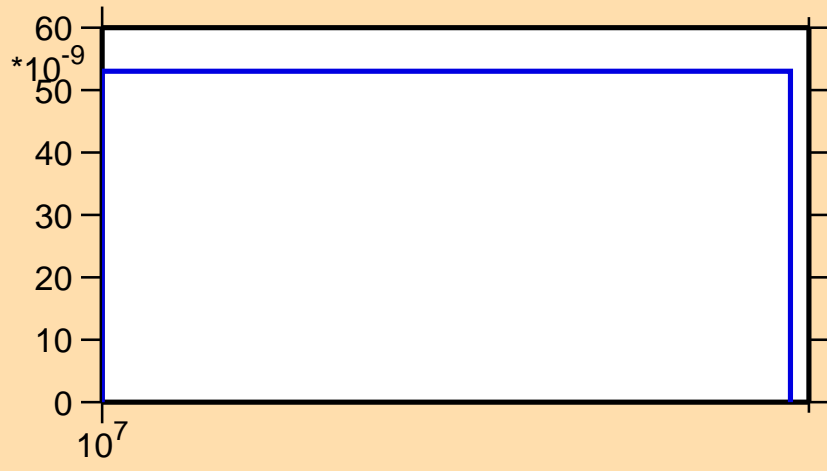
\sigma vs. E for ^{93}\text{Rh} (mt 45)
