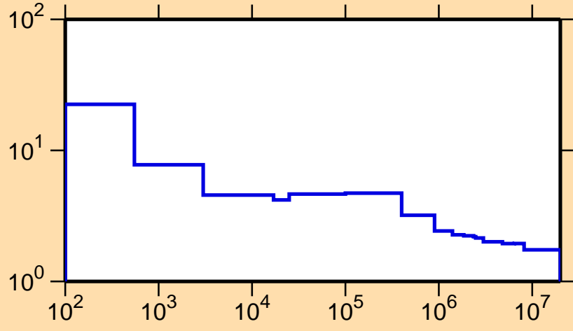
\sigma vs. E for ^{93}\text{Rh}(n,\text{nonel.})
