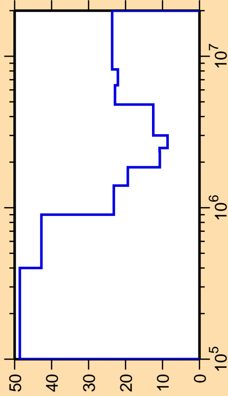
\Delta\sigma/\sigma vs. E for ^{93}\text{Rh}(n,\text{inel.})
