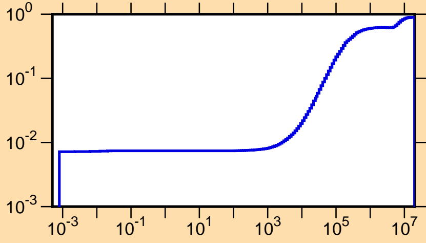
\mu vs. E for ^{94}\text{Rh}(\text{mt251})
