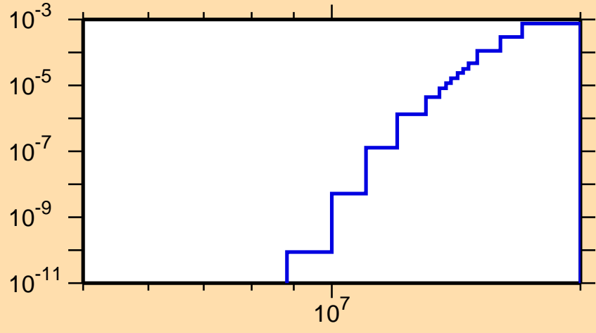
\sigma vs. E for ^{94}\text{Rh}(n,n\alpha)
