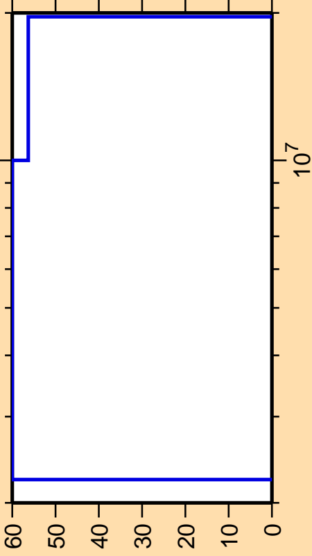
\Delta\sigma/\sigma vs. E for ^{94}\text{Rh}(n,n\text{cont.})
