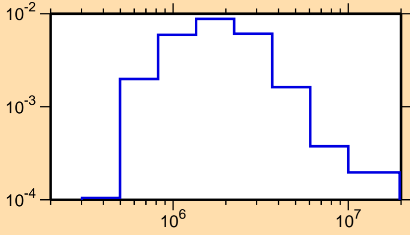
\sigma vs. E for ^{94}\text{Rh}(n,n_2)
