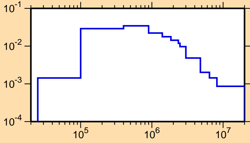
\sigma vs. E for ^{94}\text{Rh}(n,n_1)
