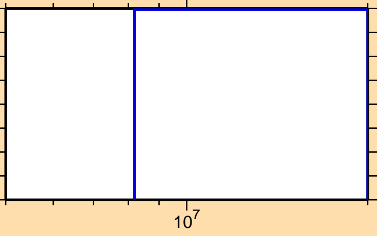
\sigma vs. E for ^{94}\text{Rh}(n,\text{pt})
