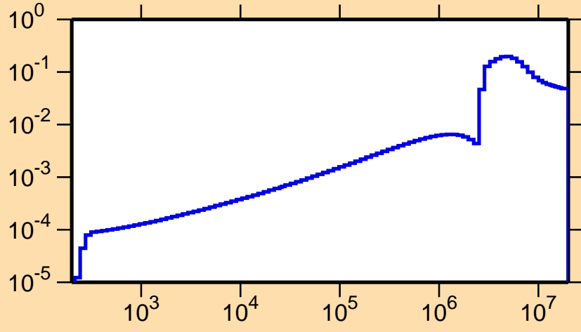
\sigma vs. E for ^{94}\text{Rh}(n,\text{inel.})
