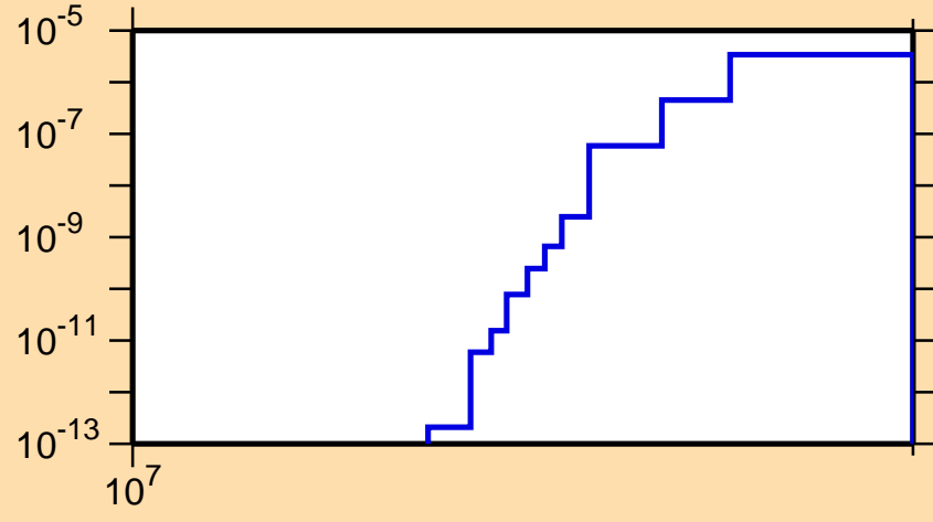
\sigma vs. E for ^{94}\text{Rh}(n,\text{nd})
