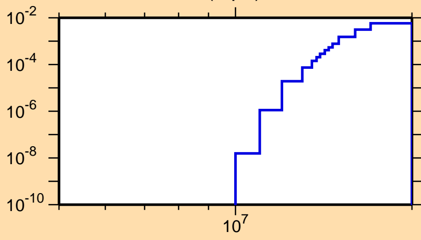
\sigma vs. E for ^{94}\text{Rh}(n,\text{pd})
