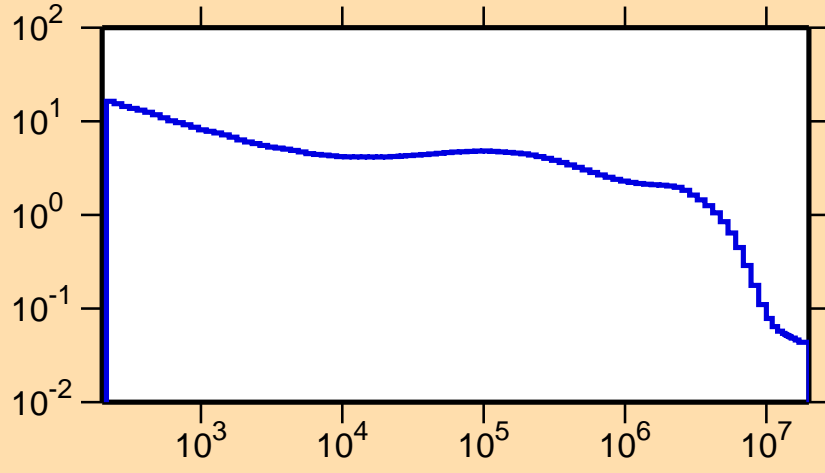
\sigma vs. E for ^{94}\text{Rh}(n,p)
