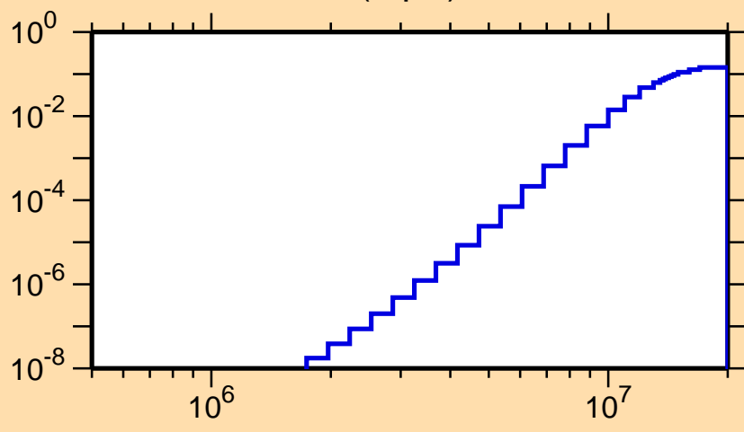
\sigma vs. E for ^{94}\text{Rh}(n,p\alpha)
