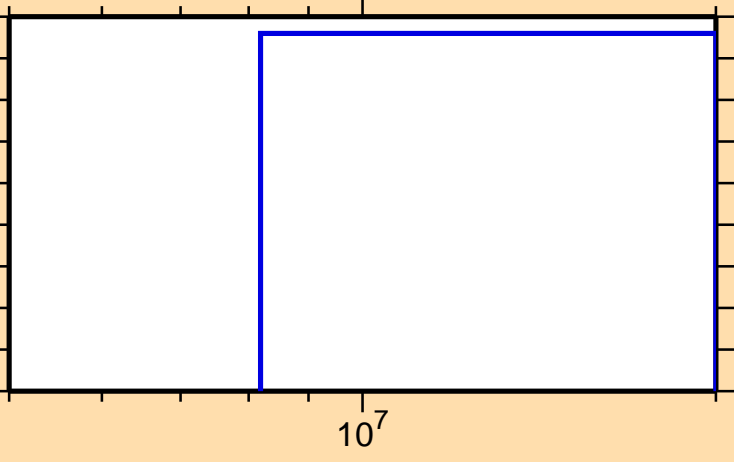
\sigma vs. E for ^{94}\text{Rh}(n,2n)
