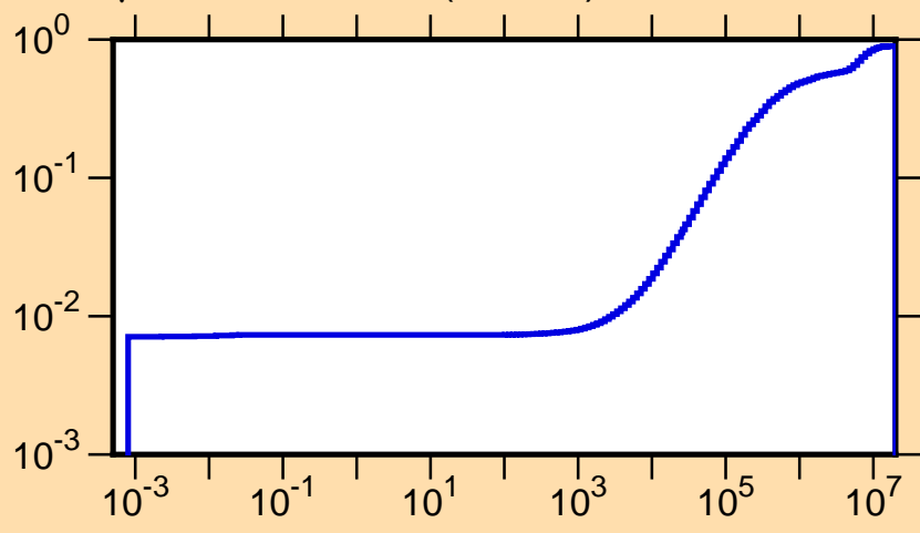
\mu vs. E for ^{95}\text{Rh}(\text{mt251})
